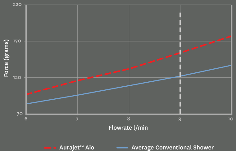
TOTAL FORCE GENERATED BY SPRAY
